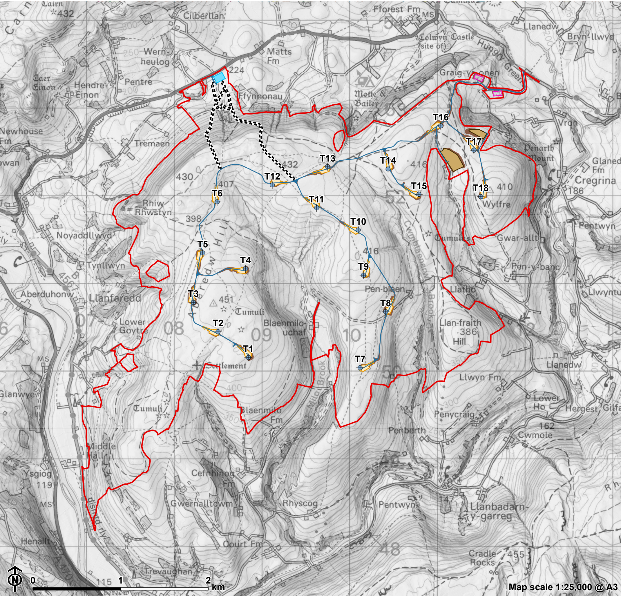
Figure 4.1a: Infrastructure Layout
