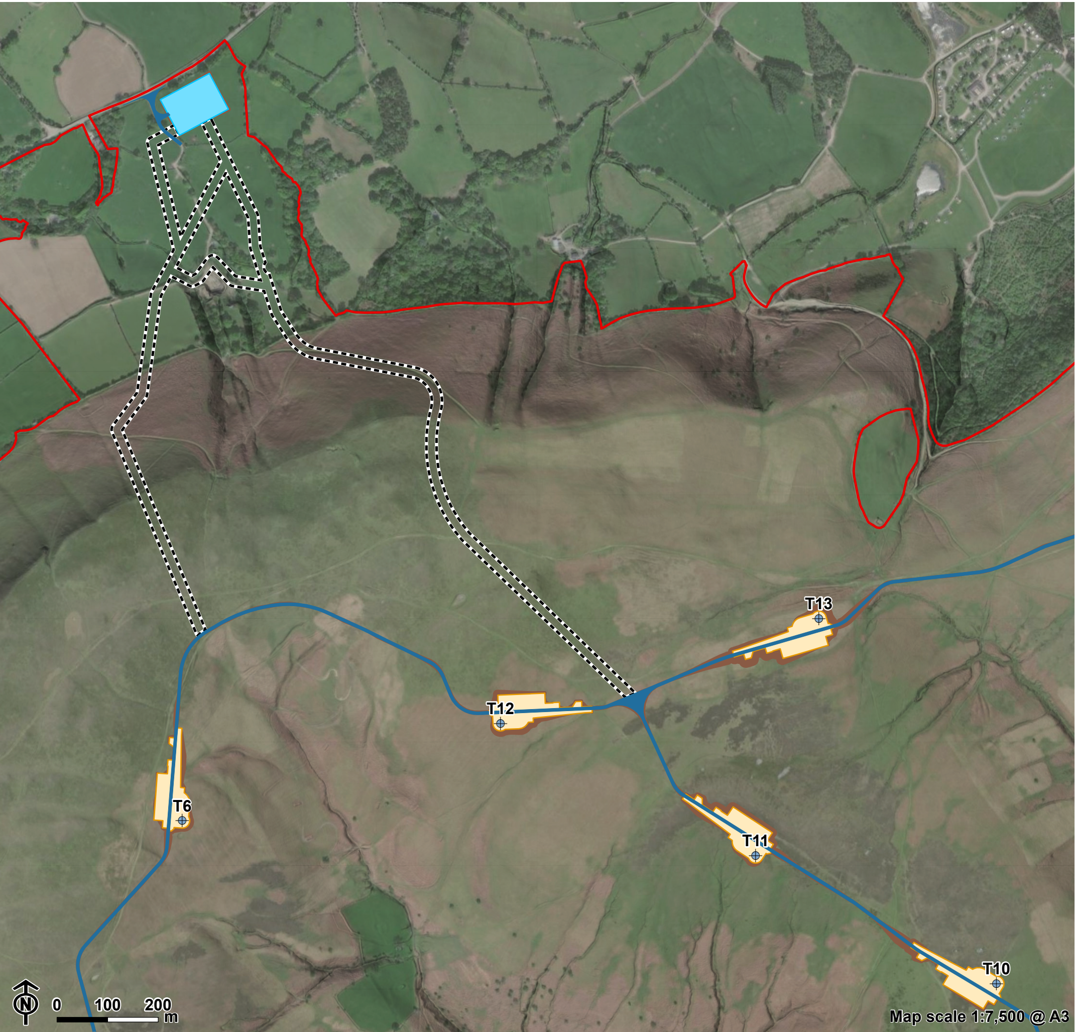
Figure 4.1c: Detailed Infrastructure Layout
