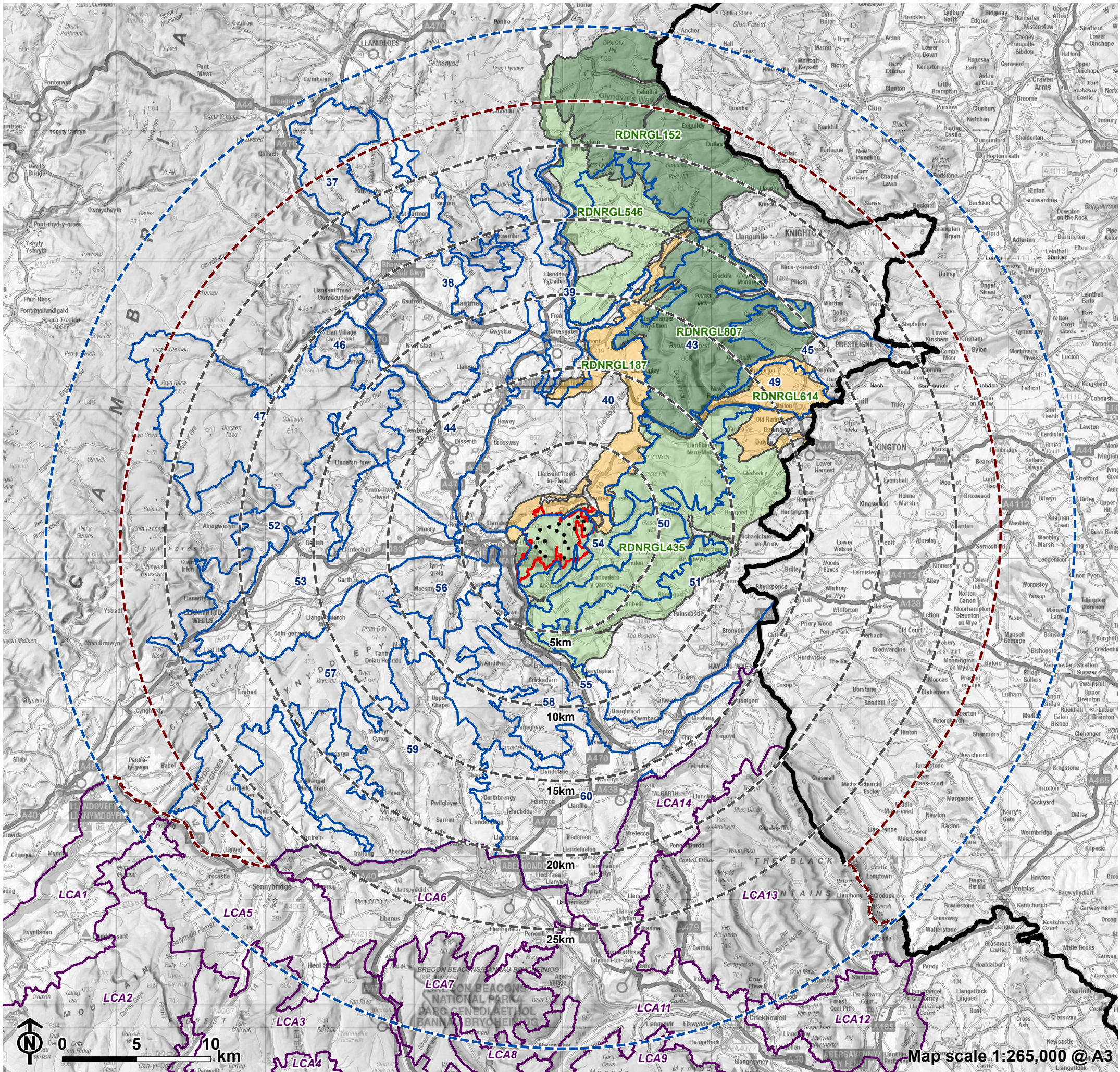
Figure 5.11c: Filtered in LANDMAP Aspect Areas - Geological Landscape (GLAA) and Landscape Units
