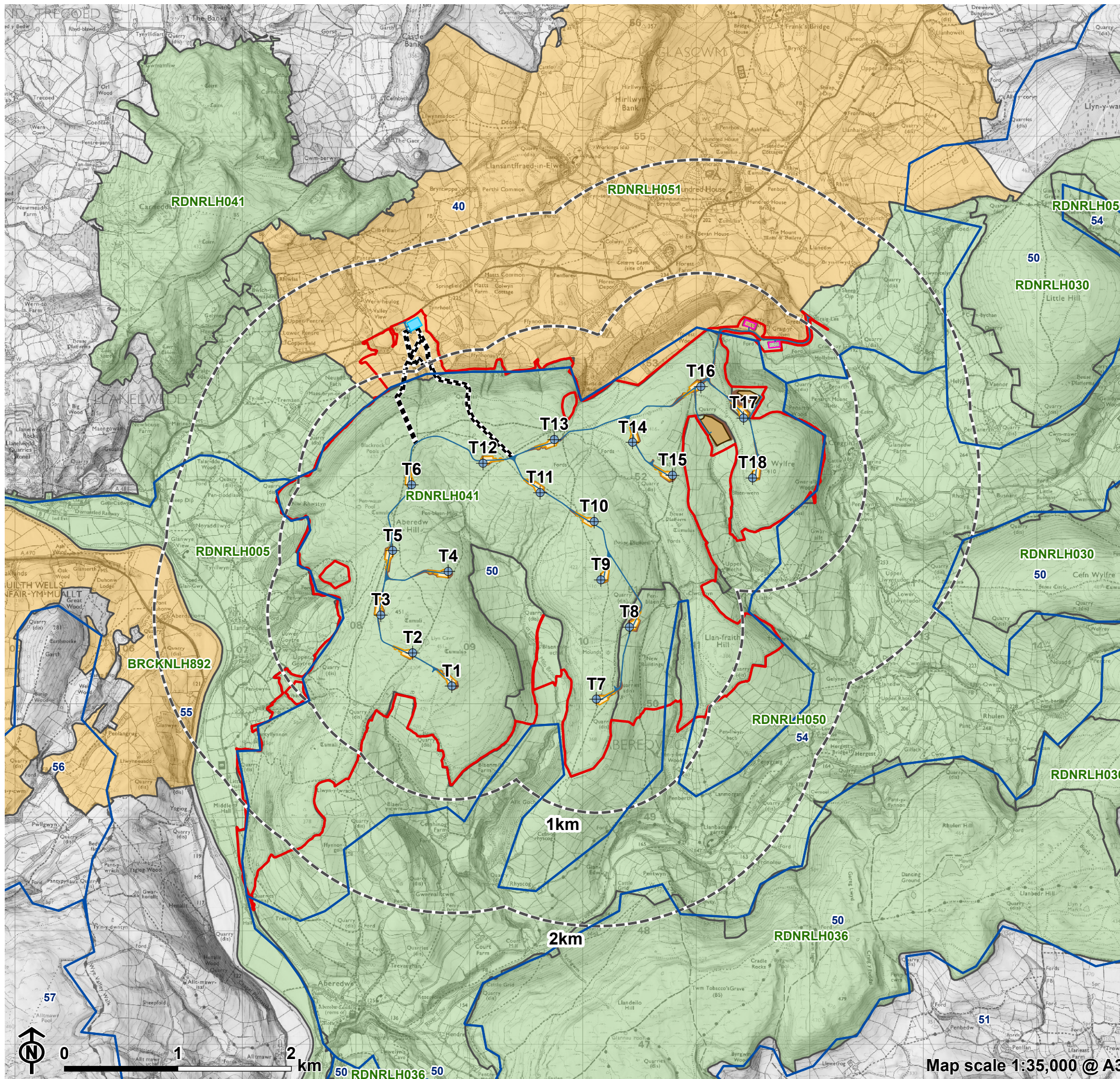
Figure 5.11d: Filtered in LANDMAP Aspect Areas - Landscape Habitats (LHAA) and Landscape Units
