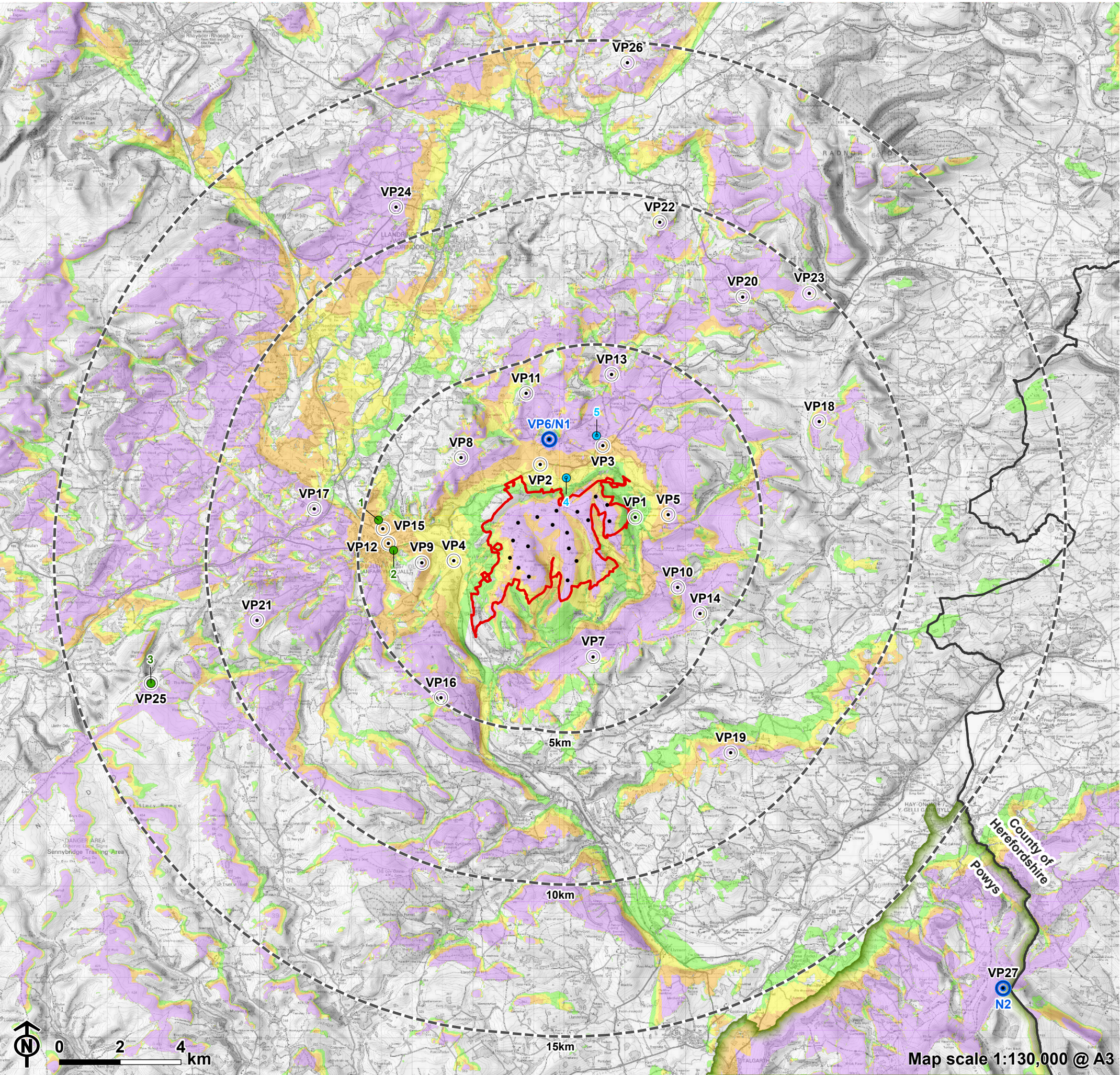
Figure 5.17b: Blade Tip Height (200m) Zone of Theoretical Visibility (15km) - Visitor Attractions and Campsites
