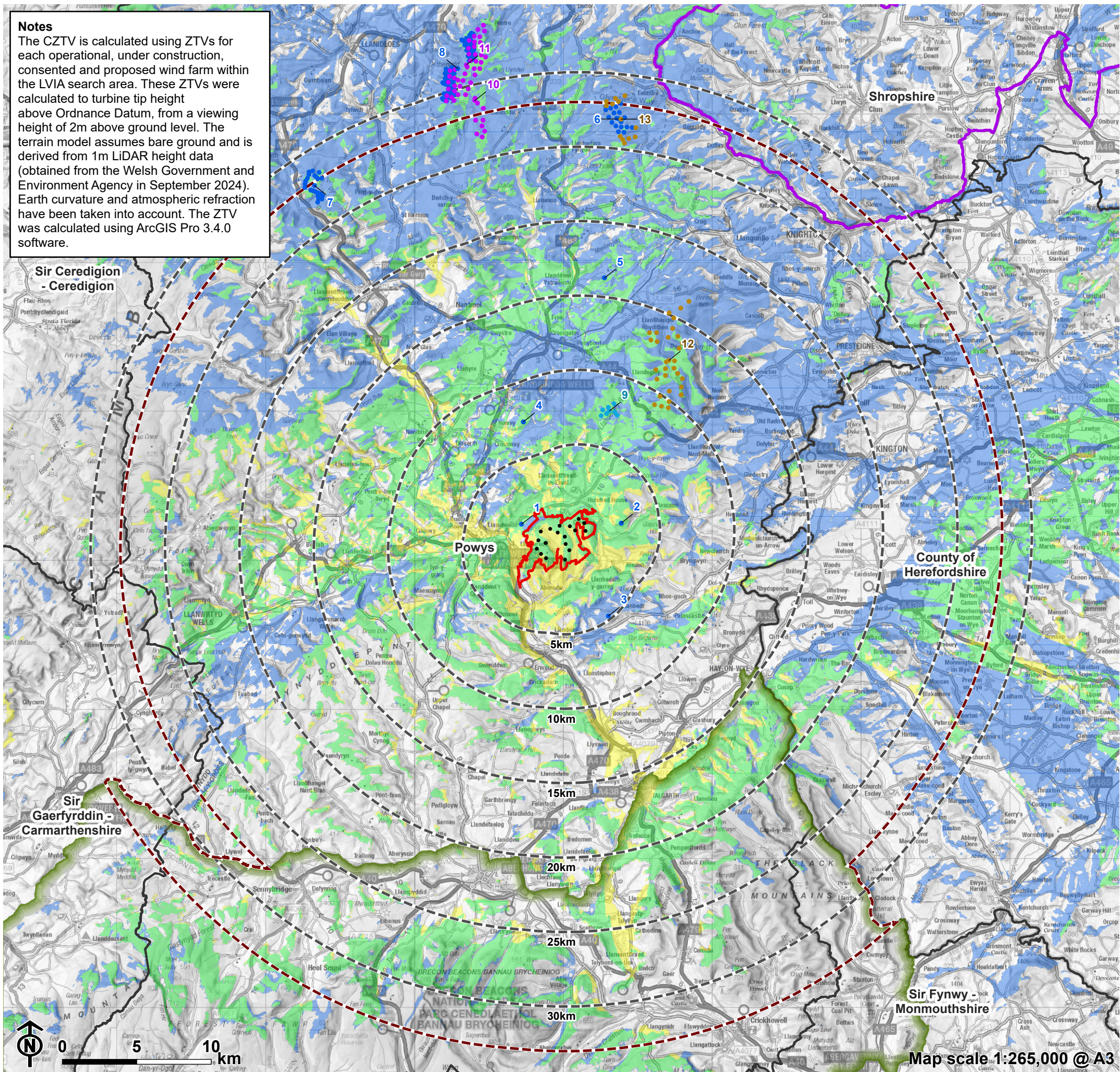
Figure 5.22: Cumulative Zone of Theoretical Visibility (CZTV) - Operational / Under Construction, Consented and Proposed Wind Farms and Aberedw Energy Park - Scenario B
