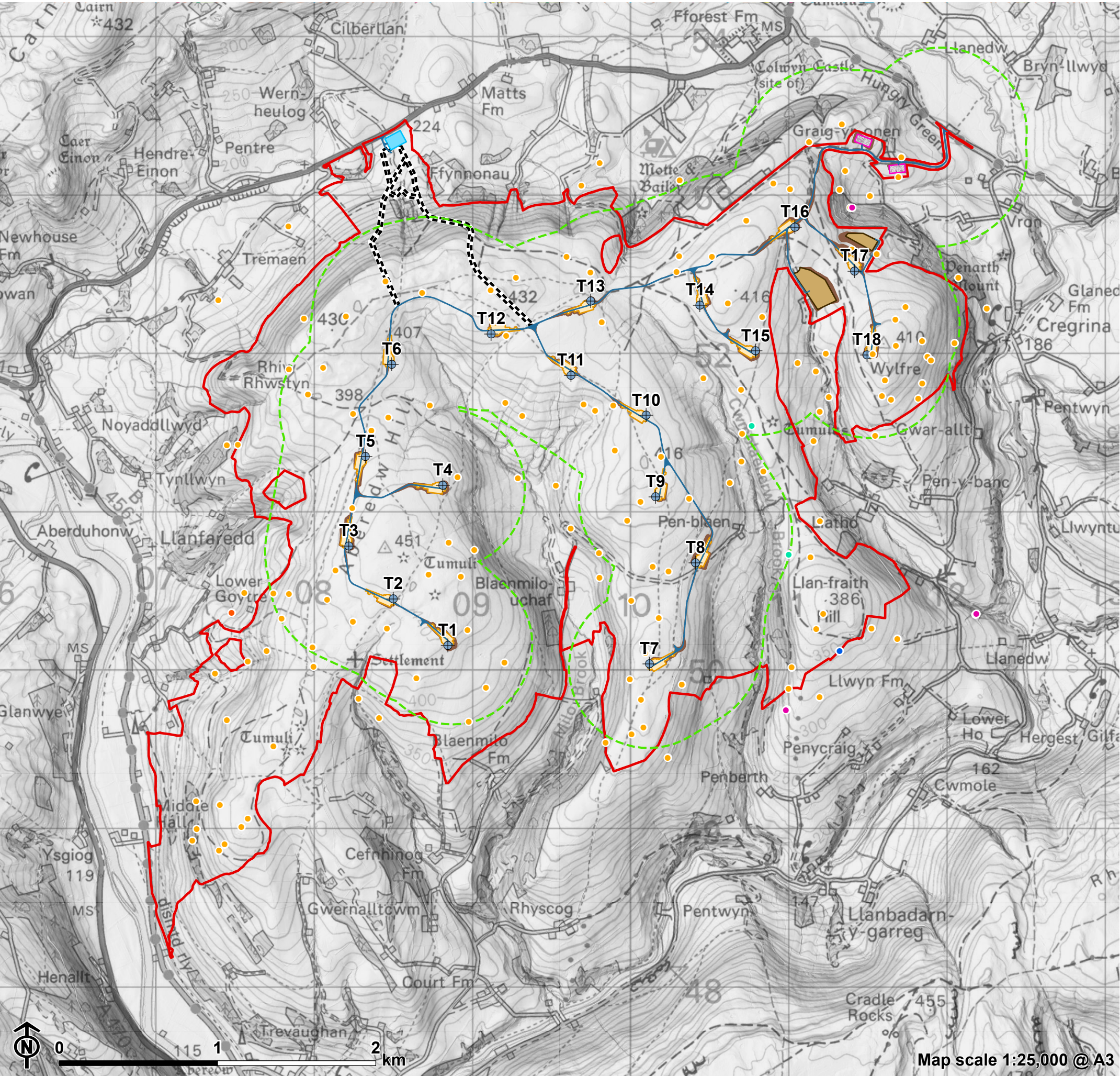
Figure 8.8: Breeding Bird Survey Results 2020
