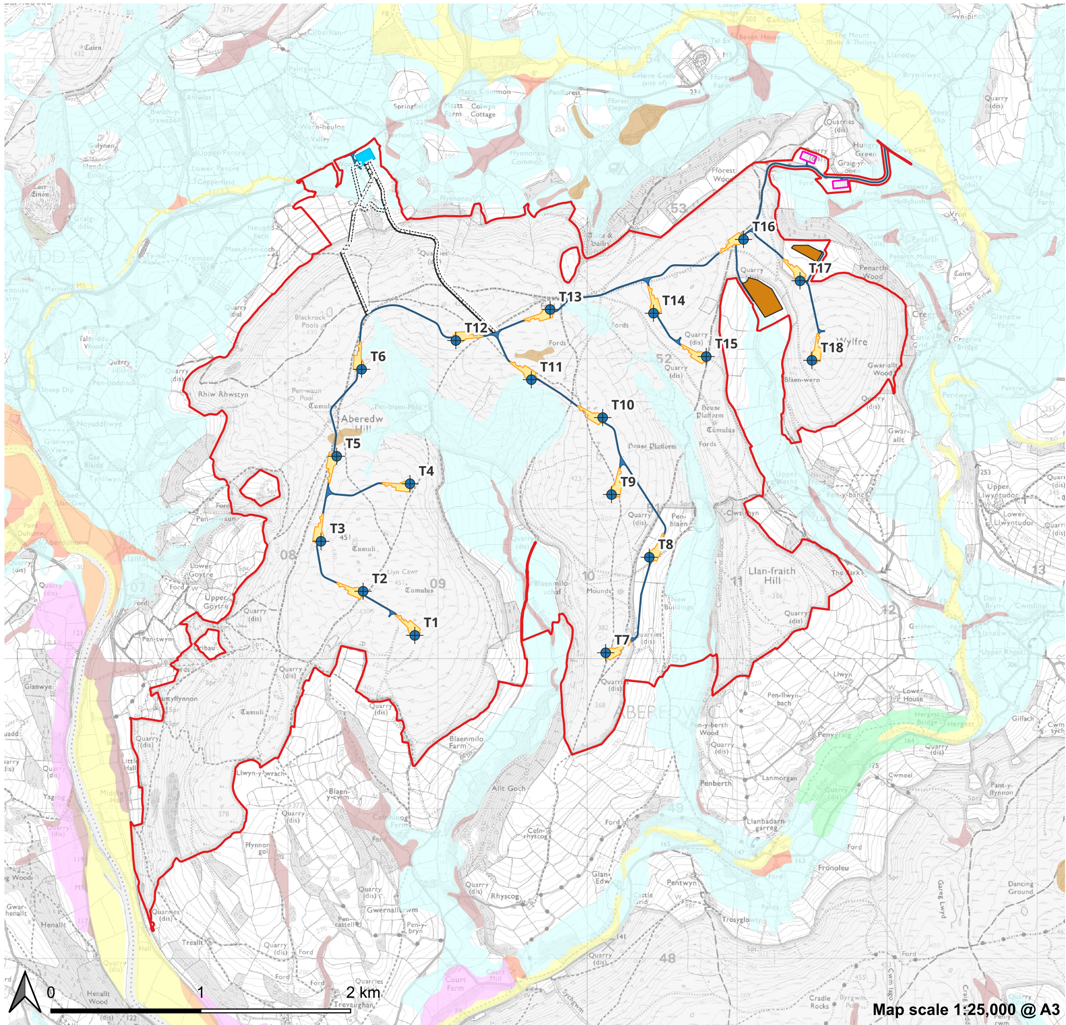
Figure 9.6: Superficial Geology
