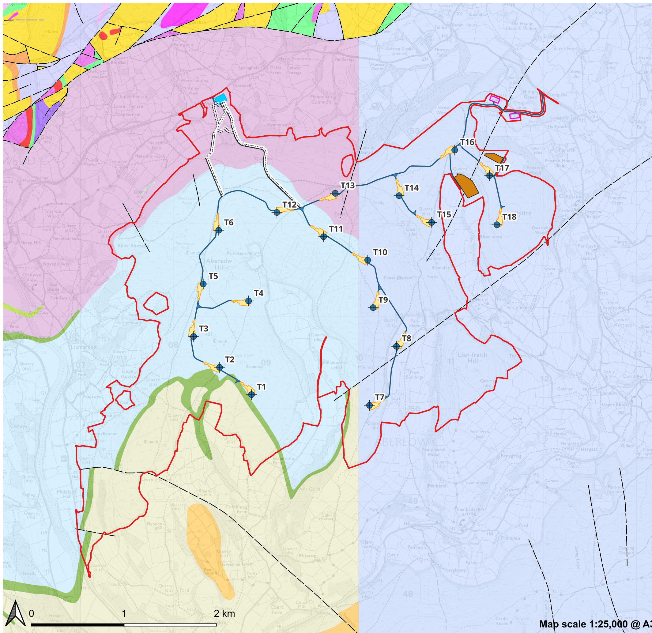
Figure 9.7: Bedrock Geology
